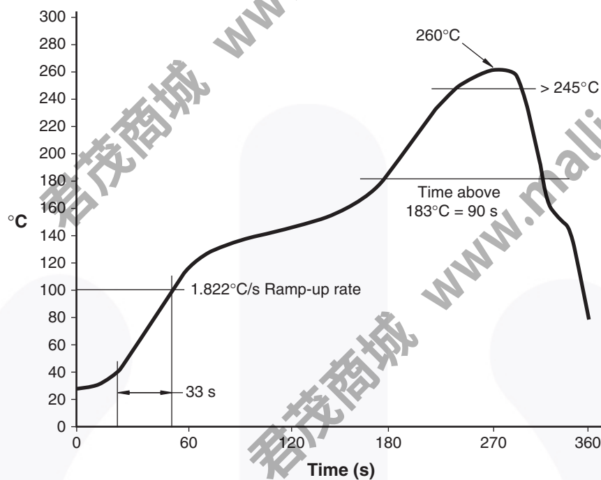
Figure 14. Reflow Profile
