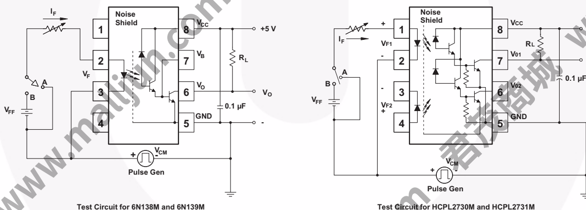
Test Circuit for 6N138M and 6N139M
