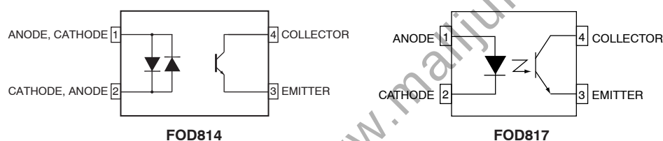
Figure 1. Schematic
