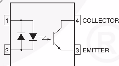
Equivalent Circuit
