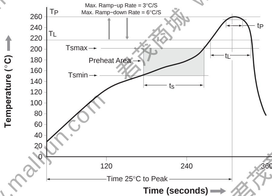
Figure 8. Reflow Profile
