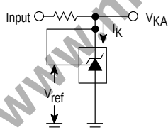
Figure 1. Test Circuit for V_{KA} = V_{\text{ref}}
