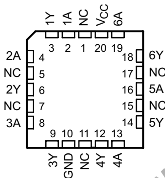
SN54HC14 . . . FK PACKAGE (TOP VIEW)
