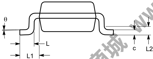
END VIEW
