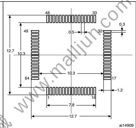
Figure 44. Recommended footprint (1)(2)
