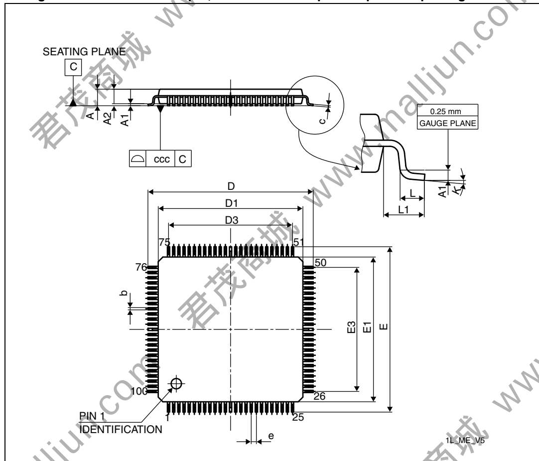
Figure 81. LQPF100 - 100-pin, 14 x 14 mm low-profile quad flat package outline
