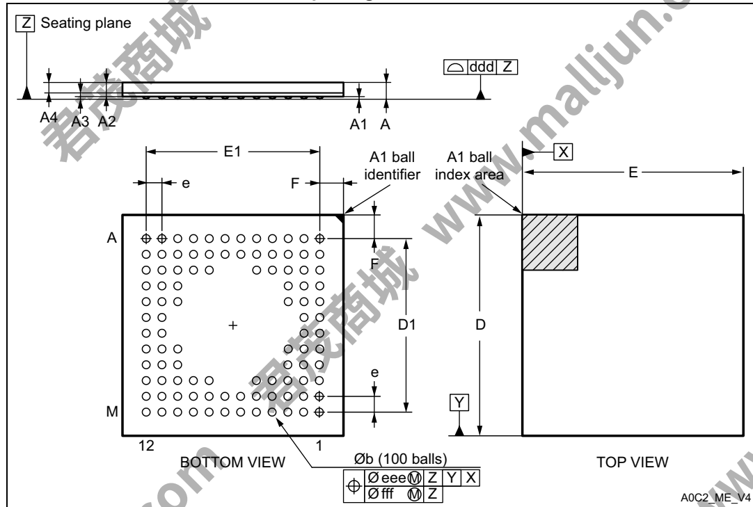
Figure 45. UFBGA100 - 100-ball, 7 x 7 mm, 0.50 mm pitch, ultra fine pitch ball grid array array package outline
