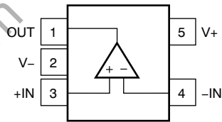
DBV Package: TLV333 5-Pin SOT23 Top View
