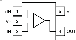
DCK Package: TLV333 5-Pin SC70 Top View
