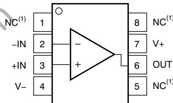
D Package: TLV333 8-Pin SOIC Top View
