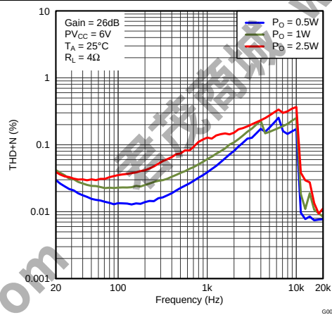
Figure 1. Total Harmonic Distortion + Noise (BTL) vs Frequency
