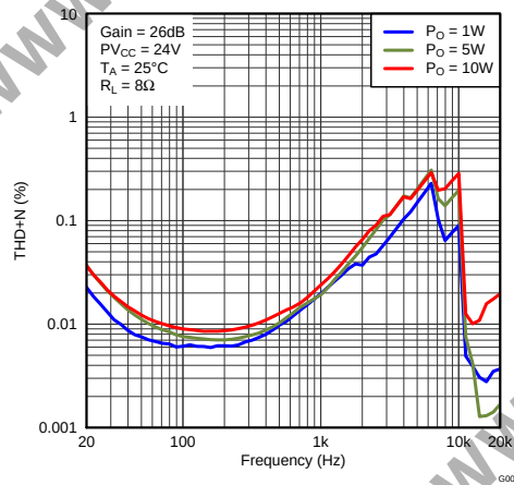
Figure 5. Total Harmonic Distortion + Noise (BTL) vs Frequency
