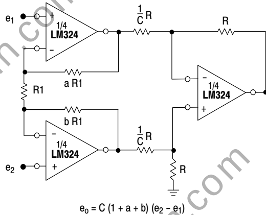
Figure 13. High Impedance Differential Amplifier
