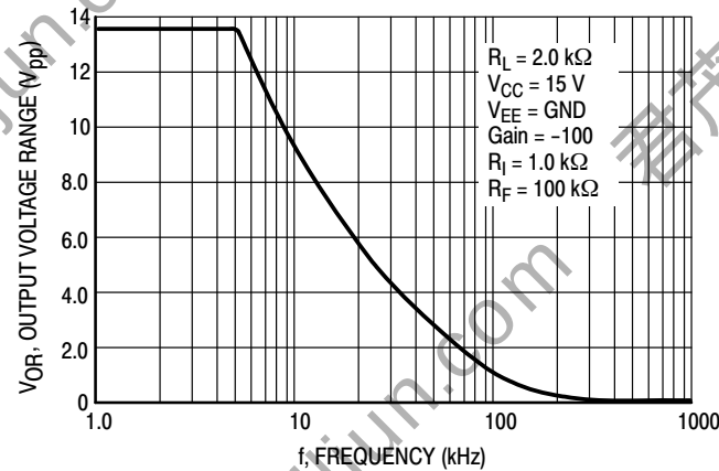
Figure 7. Large-Signal Frequency Response
