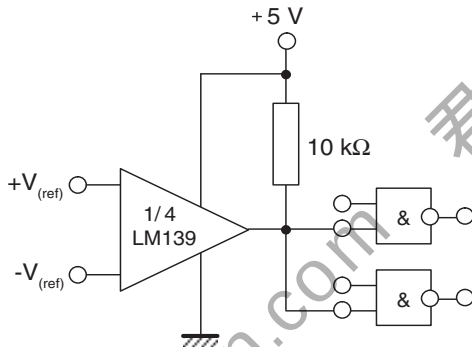
Figure 10. Driving TTL
