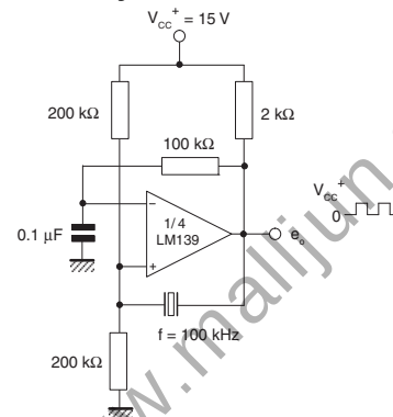
Figure 19. Crystal-controlled oscillator
