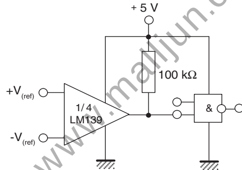
Figure 9. Driving CMOS
