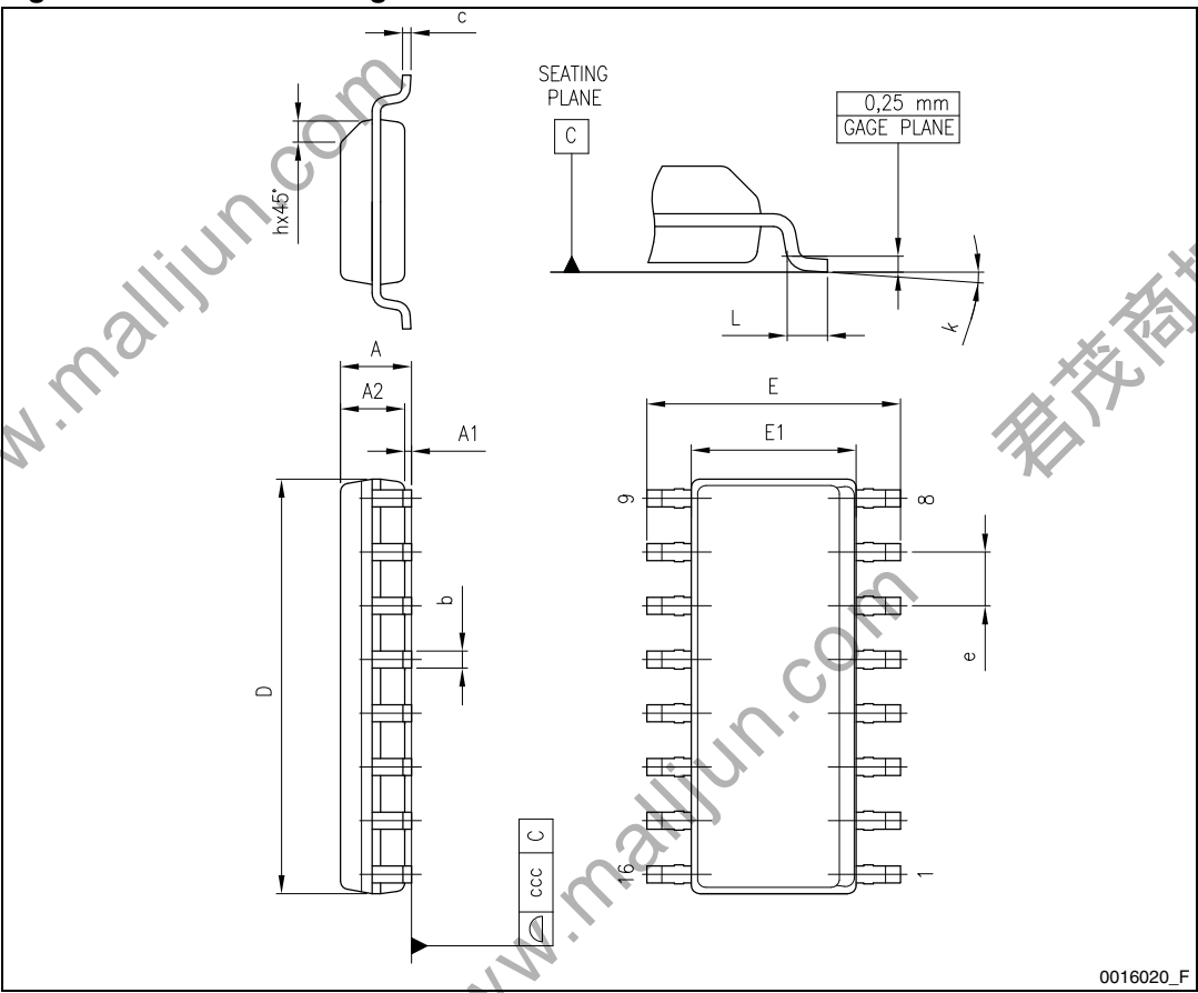
Figure 34. SO16N drawing
