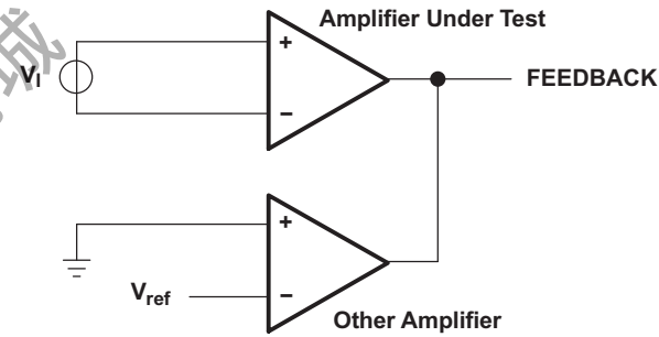
Figure 6. Amplifier Characteristics
