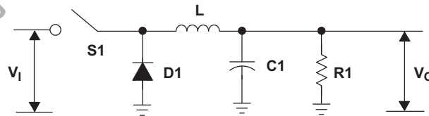
Figure 14. Switching Circuit
