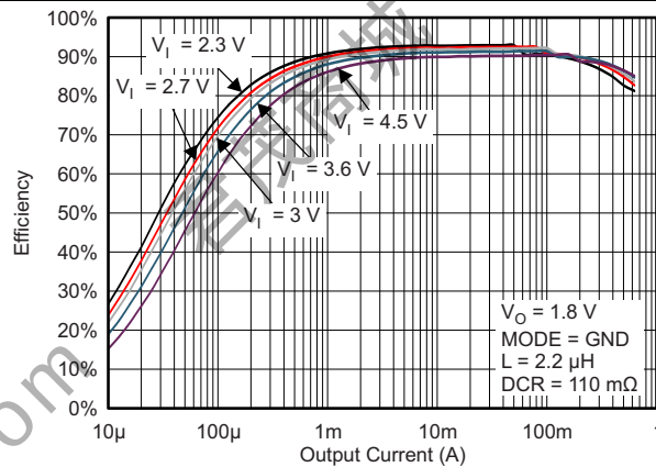
Figure 7. Efficiency (Power Save Mode) vs Output Current
