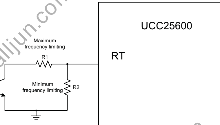
Figure 20. Maximum and Minimum Frequency Setting for UCC25600
