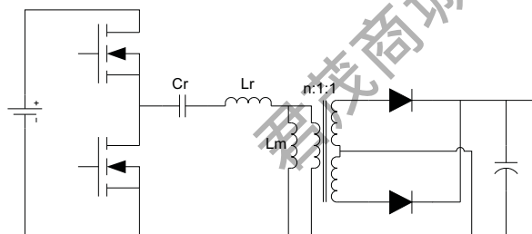
Figure 14. LLC Resonant Converter
