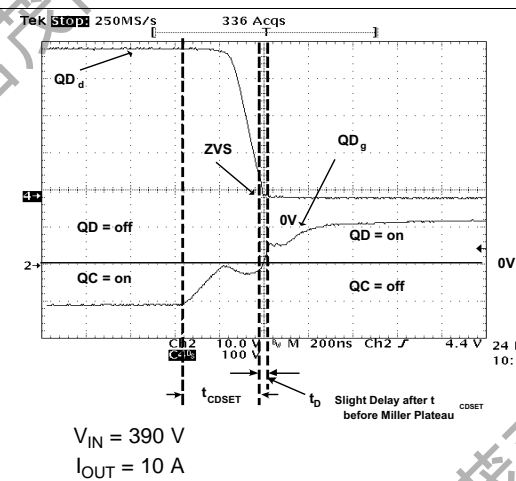
Figure 60. Full-Bridge Gate Drives and Switch Nodes (QD g QD d )
