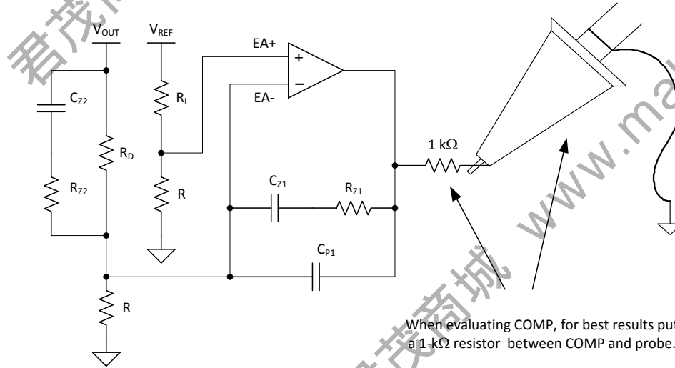
Figure 50. Type 3 Compensation Evaluation
