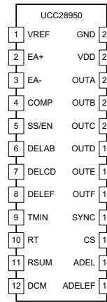
Pin Functions
