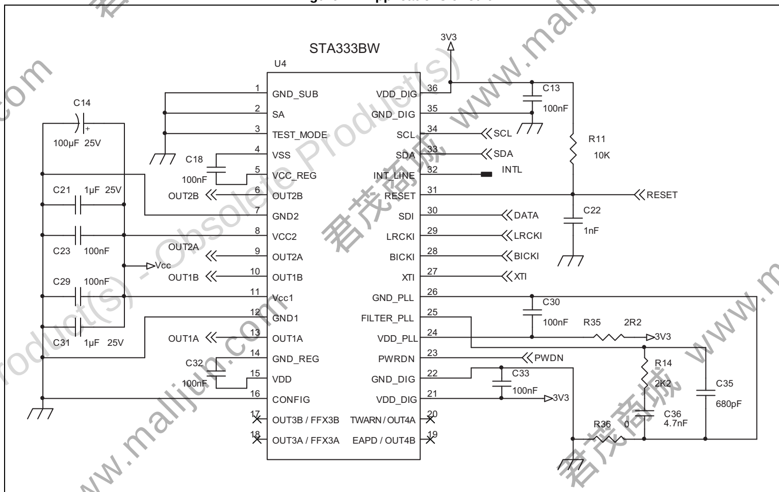
Figure 21. Applications circuit
