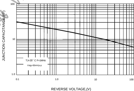
FIG.5-TYPICAL JUNCTION CAPACITANCE
