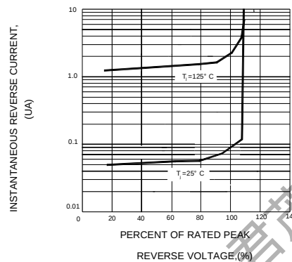
FIG.4-TYPICAL REVERSE CHARACTERISTICS
